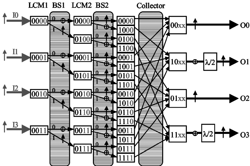
FIGURE 3 Switching network for non-blocking 4 \times 4 channels optical switch.
