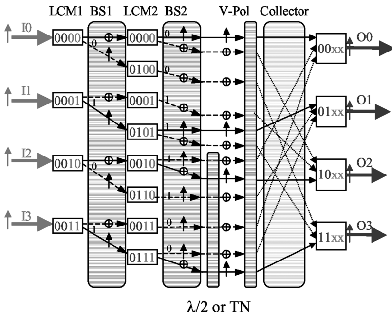
FIGURE 7 Polarization states and crosstalk cleaning in blocking 4 \times 4 channels optical switch.
