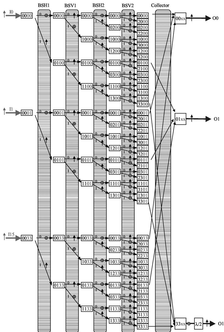
FIGURE 6 Switching network for non-blocking 16 × 16 channels optical switch.
